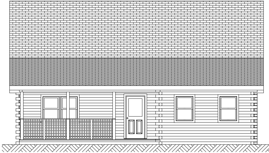
Front
