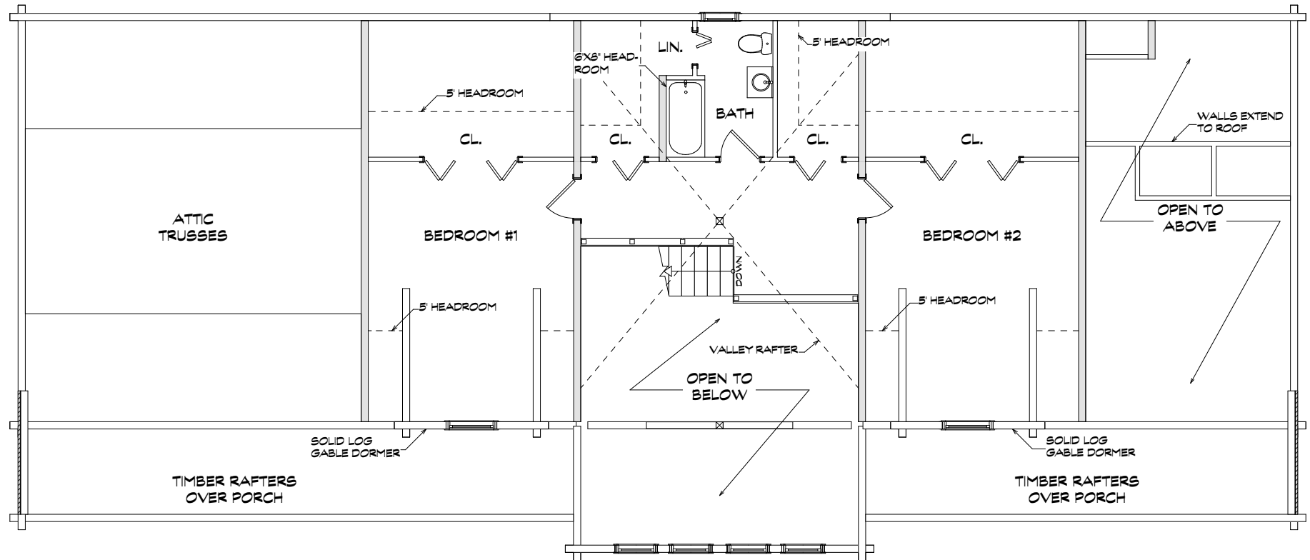
Second Floor
